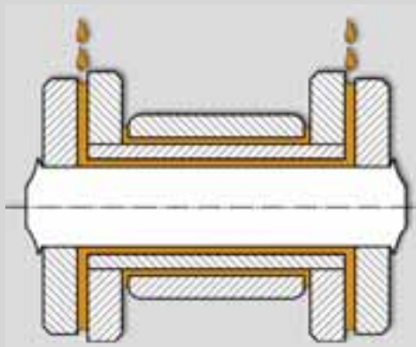
Fig. 2: Cross-section of a chain link
